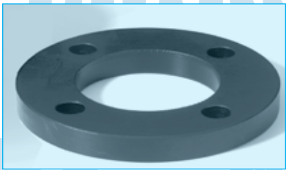
AKZO flange drilled according to DIN 2501 PN 10 DN 50 (fits behind abovementioned flanged bush)
