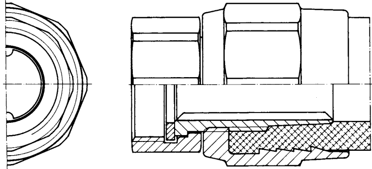
Sleeve couplings type HGF
